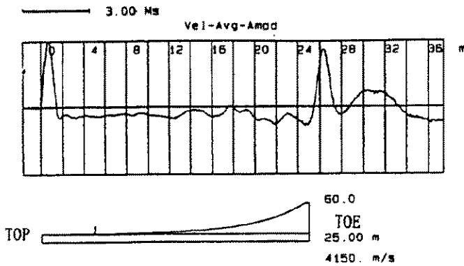
FIG. 3(a) Typical Velocity Record Indicating Pile of Generally Uniform Nature (Gradual Impedance Changes or Soil Friction)
