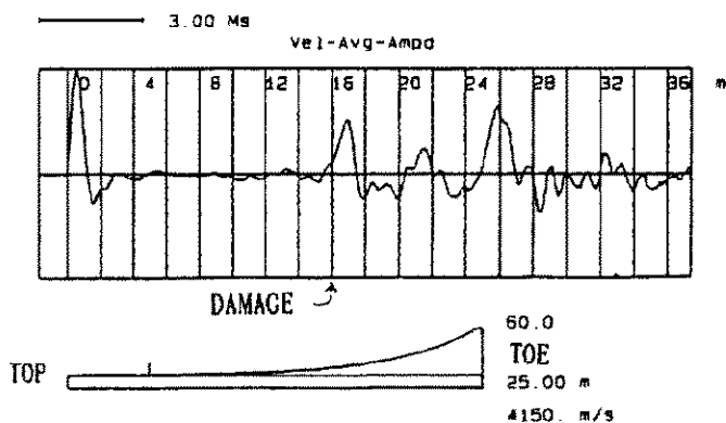
FIG. 3(b) Typical Velocity Record Indicating Major Changes in Impedance (Severe Damage or a Cracked Pile)
